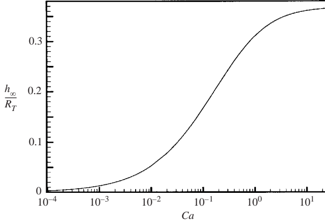
FIGURE 15. Dimensionless film thickness, h_\infty/R_T , behind a semi-infinite air finger propagating into a fluid-filled rigid circular tube of radius R_T vs. capillary number.
